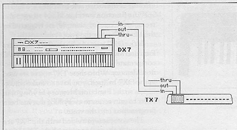
Basic MIDI connections for using a TX7 tone generator with a DX7 synthesizer.
