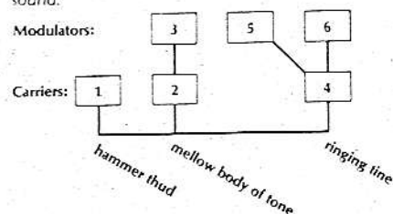
Fig. 3. Algorithm 26 being used for electric piano sound.
